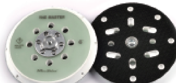
3011150 6" (150mm) Max OPM: 12000 Thread: 5/16"-24 Hole: 8
