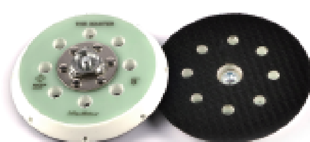
3011125 5" (125mm) Max OPM: 12000 Thread: 5/16"-24 Hole: 8
