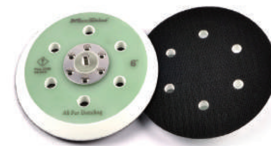
3013150 6" (150mm) Max OPM: 12000 Thread: 5/16"-24 Hole: 6
