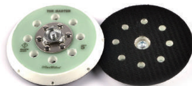
3011125P 5" (125mm) Max OPM: 12000 Thread: 5/16"-24 Hole: 8
