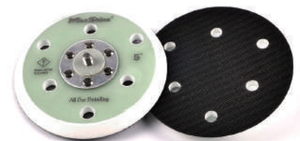
3013125 5" (125mm) Max OPM: 12000 Thread: 5/16"-24 Hole: 6
